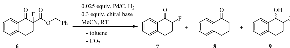
Scheme 3. Reaction of benzyl 2-fluoro-1-tetralone-2-carboxylate 6 .
