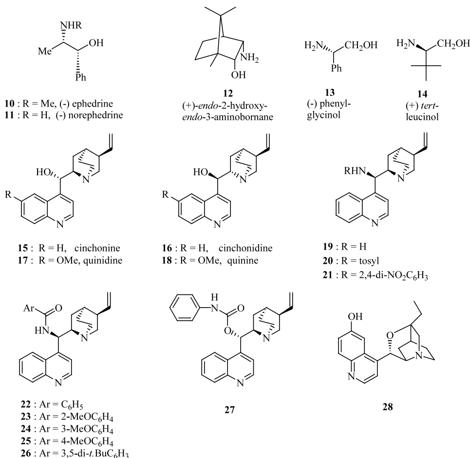
Figure 1. Chiral bases used as inducers.
