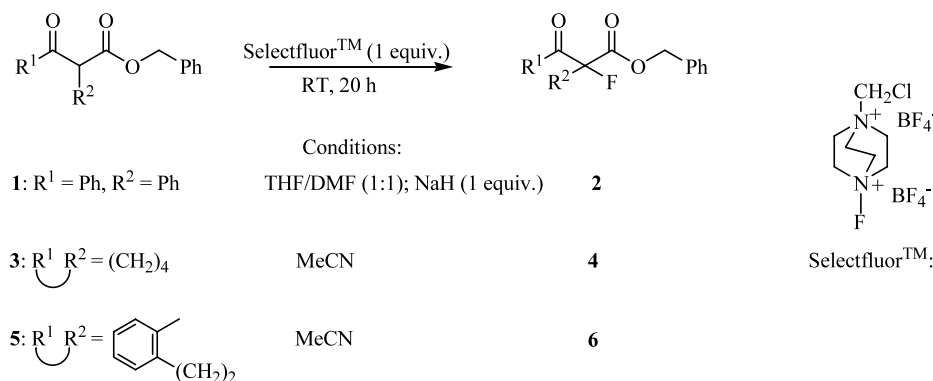
Scheme 2. Electrophilic fluorination of \beta -oxoesters 1 , 3 and 5 .
