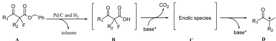
Scheme 1. The three steps of the cascade reaction.
